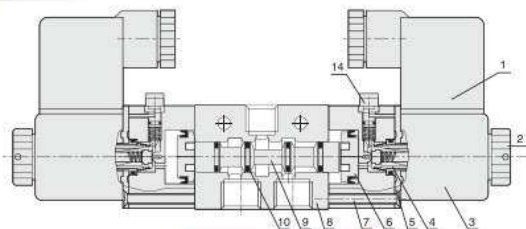
Double solenoid valve
